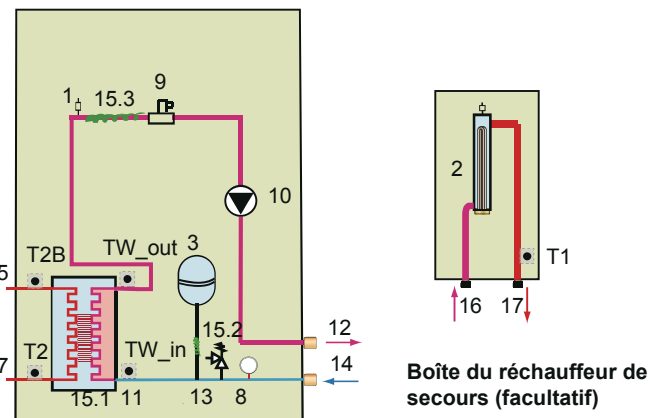
1-phase 5/7/9 kW
