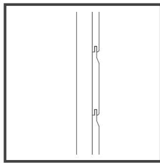
Shiplap Cladding
