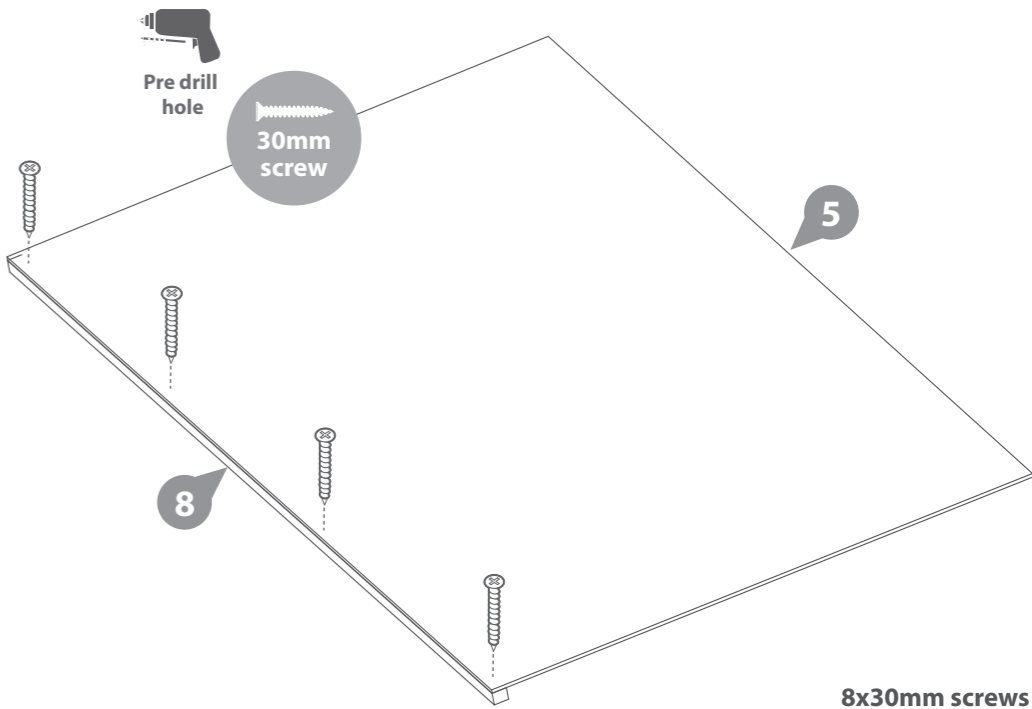
8x30mm screws
