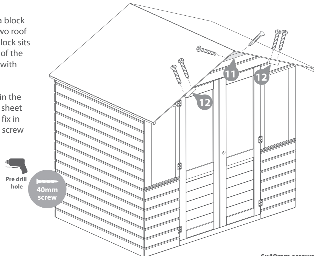
6x40mm screws
