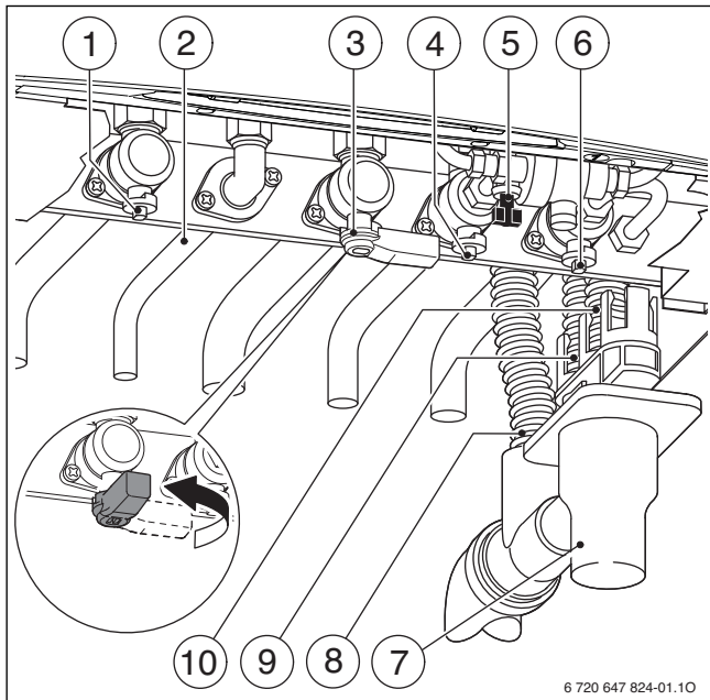
Fig. 1 Raccordements
