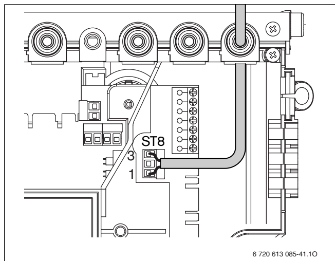
Fig. 43 Raccord thermostat
