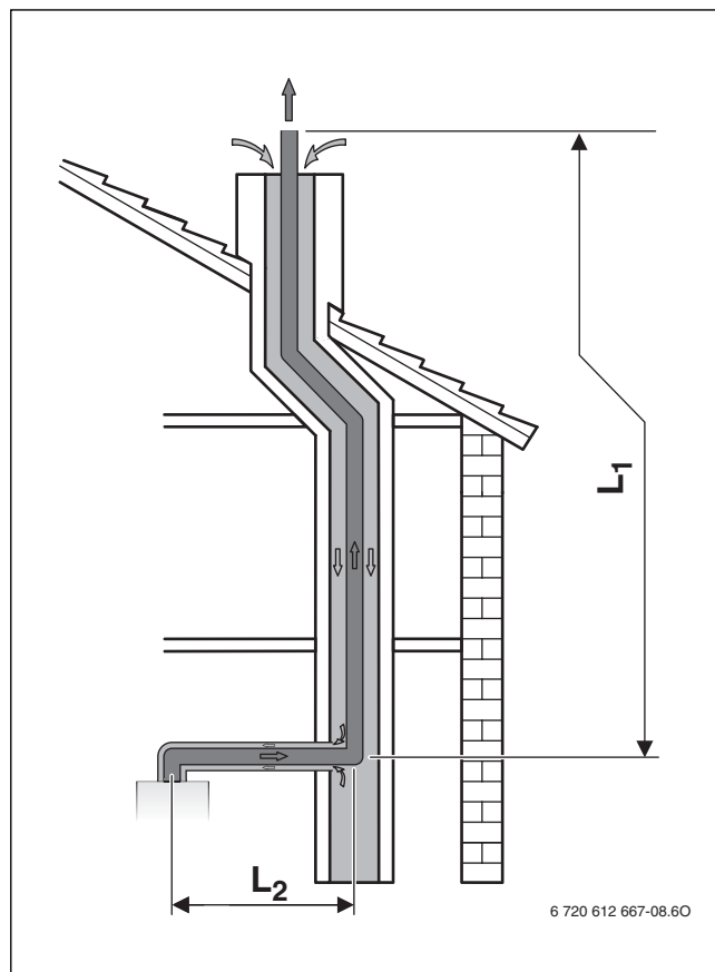
Fig. 18 Configuration C 93
