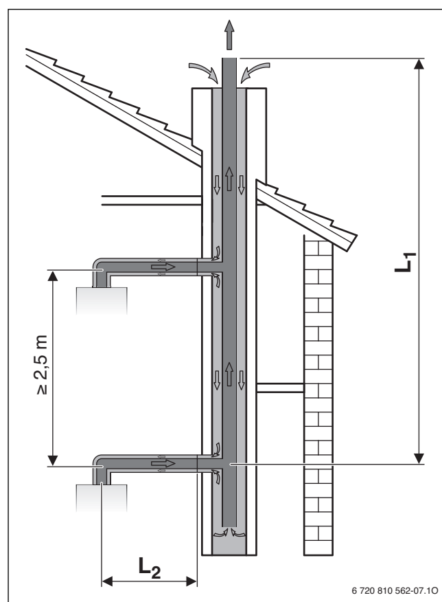
Fig. 22 Configuration C 43
