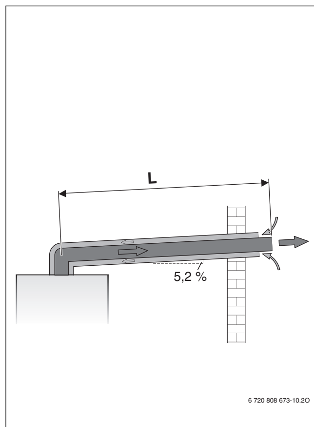
Fig. 21 Configuration C 13
