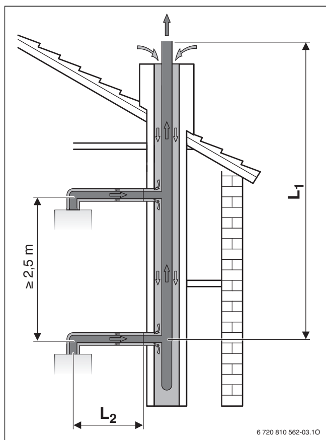
Fig. 23 Configuration C 43p
