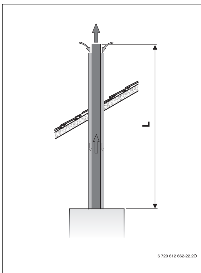
Fig. 20 Configuration C 33
