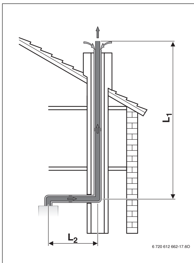
Fig. 19 Configuration C 33
