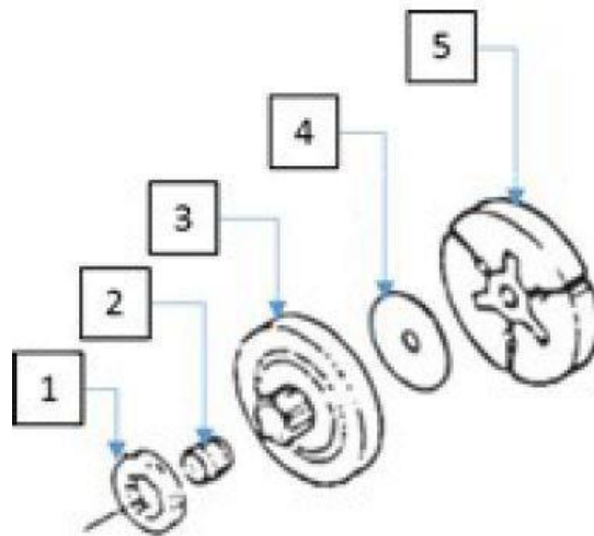
1. Sprocket 2. Needle bearing. 3. Clutch drum. 4. Spacer. 5. Clutch shoe.
