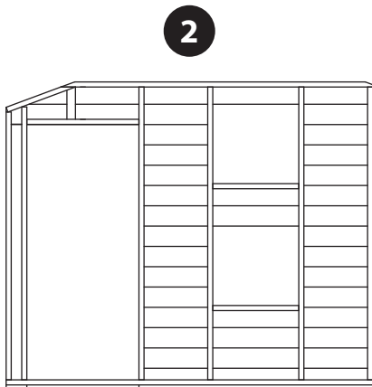
Door Panel QTY 1 AI-02S112SWLFD2020X1691-V1
