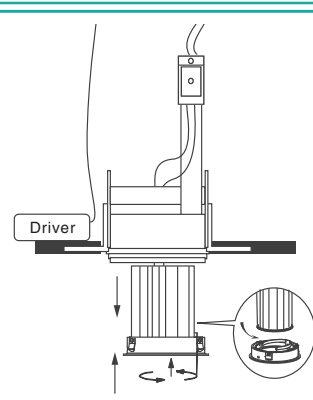
MR16 LED MODULE
