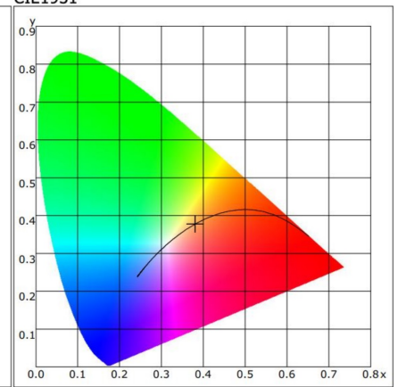
CIE1931
