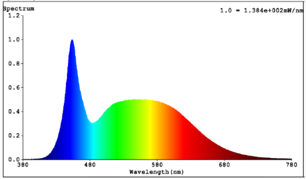
Spectral power distribution for SSL-TPL-36W-230V 6500K:
