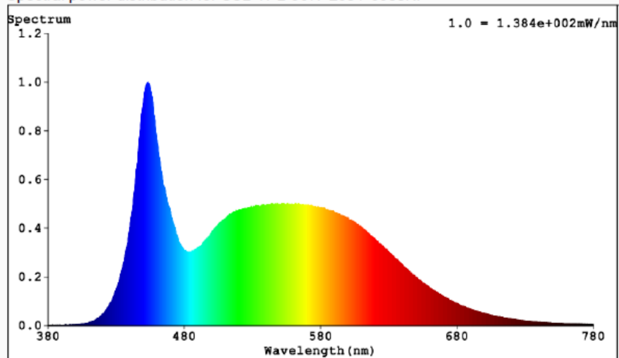
Spectral power distribution for SSL-TPL-36W-230V 6500K:
