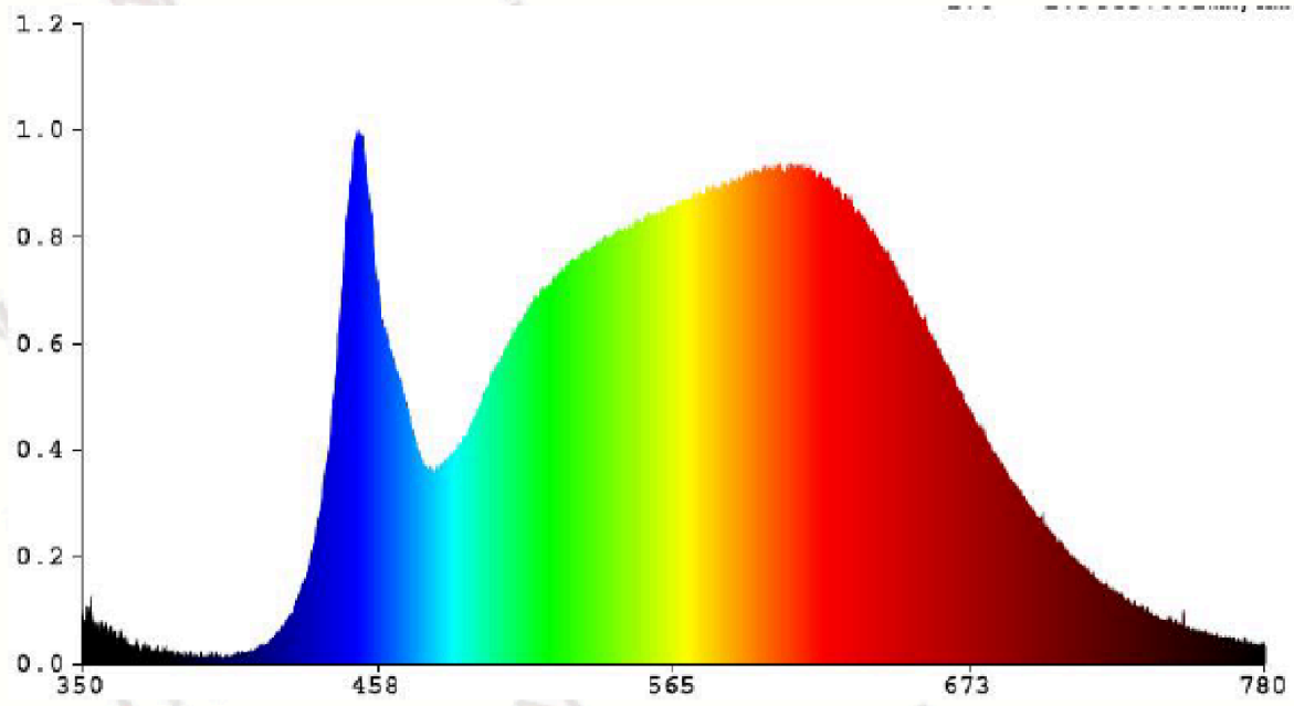
WE-SL1502W
