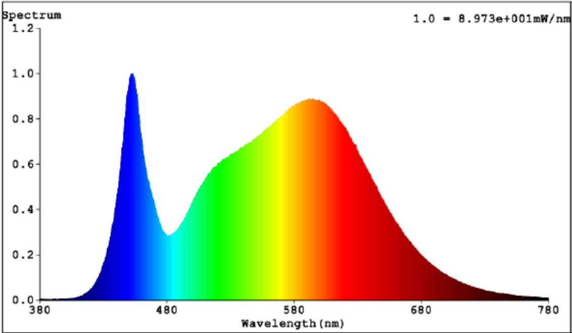
Spectral power distribution for light source of SSL-TPL-36W-230V 4000K:
