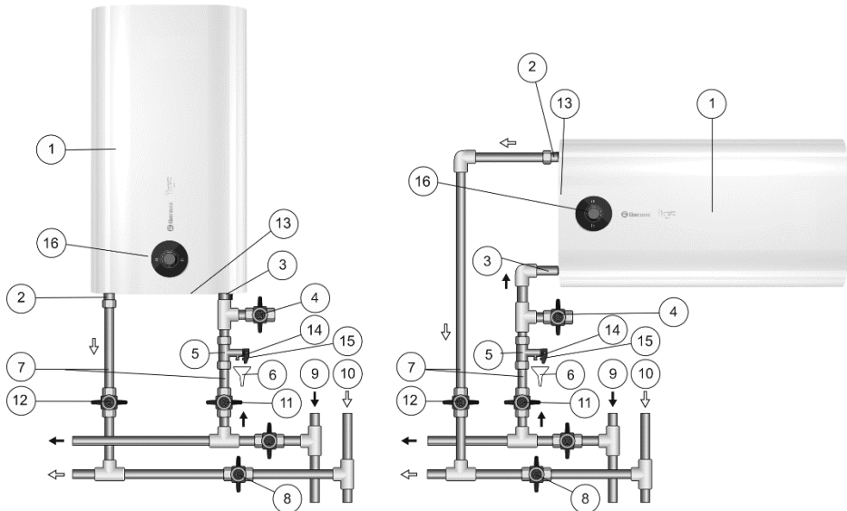
Figure 1. EWH connection diagram to water supply
