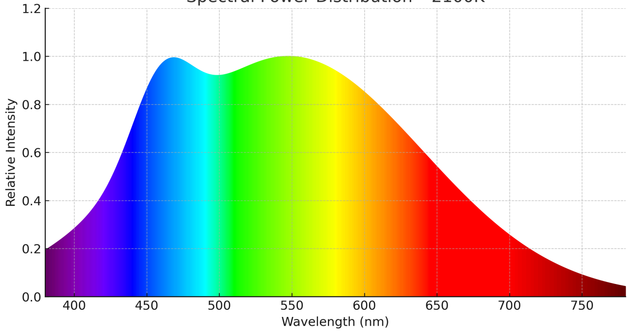
Spectral Power Distribution - 2100K
