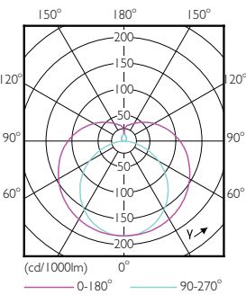
Light Distribution Diagram - MAS LEDtube HF 1200mm HE 16.5W 865 T5
