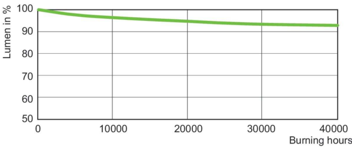
Lumen Maintenance Diagram - MST SON-T APIA Plus Xtra 400W E40 1SL/12
