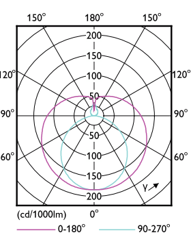
Light Distribution Diagram - MAS LEDtube VLE 1200mm UO 15.5W 865 T8
