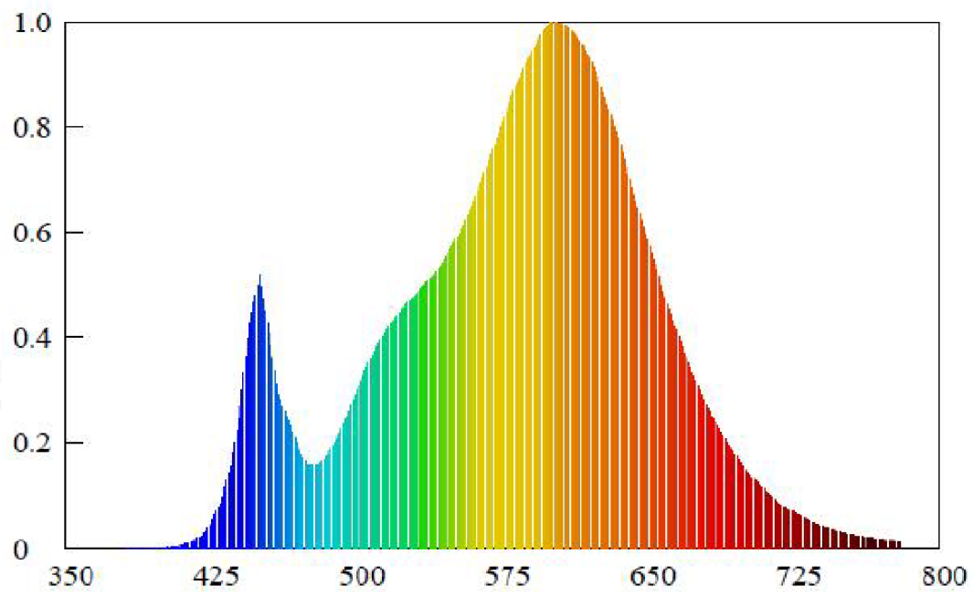
Spectral power distribution (3000K)
