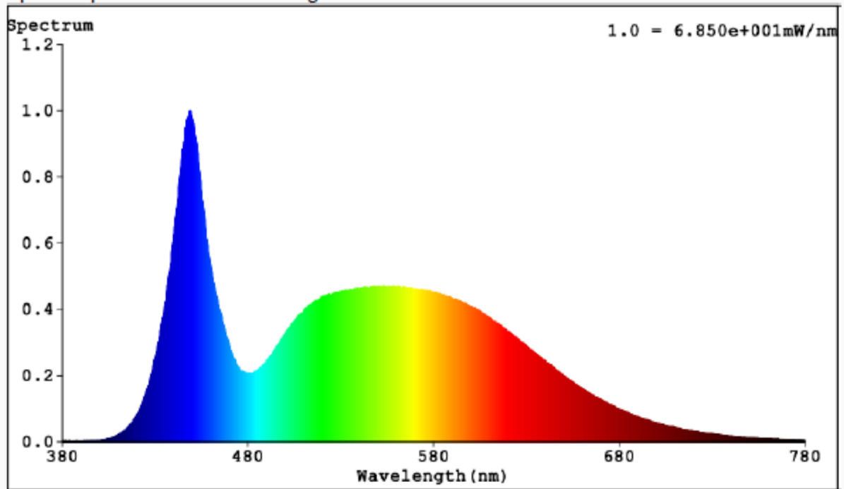
Spectral power distribution for light source of SSL-TPL-18W-230V 6500K:
