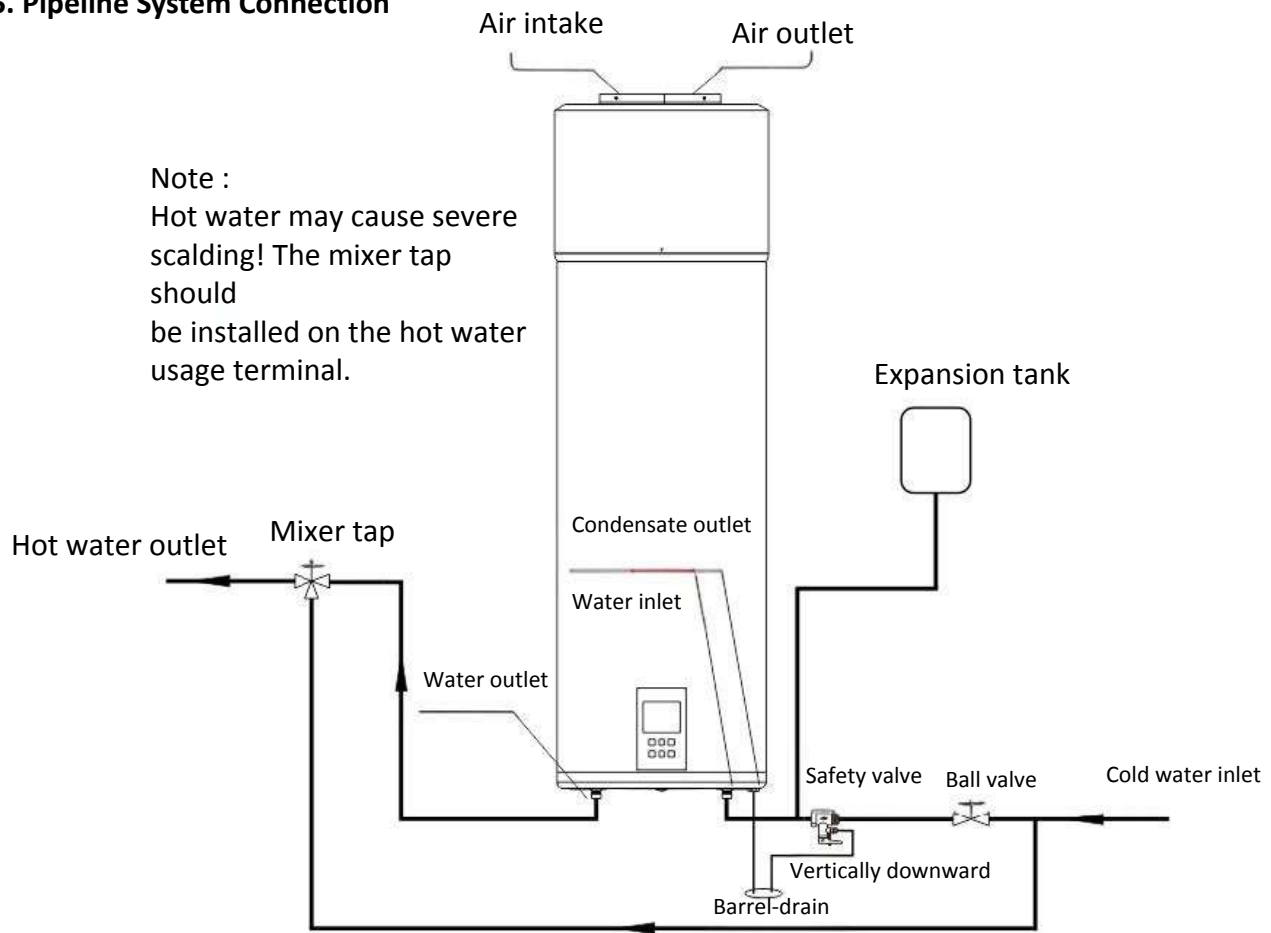
Fig.5 Pipeline system connection
