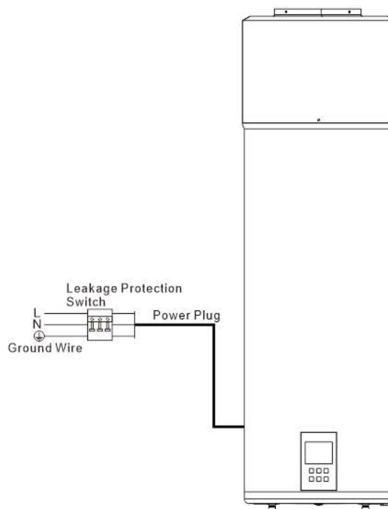
Fig.6 Earth leakage protection
