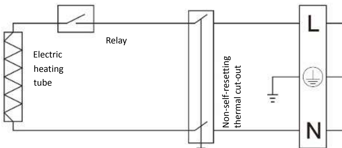
Fig.2 Working principles of electricity-assistant heating
