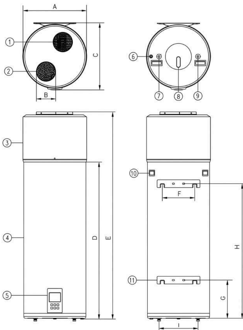
Fig.3 Appliance dimensions
