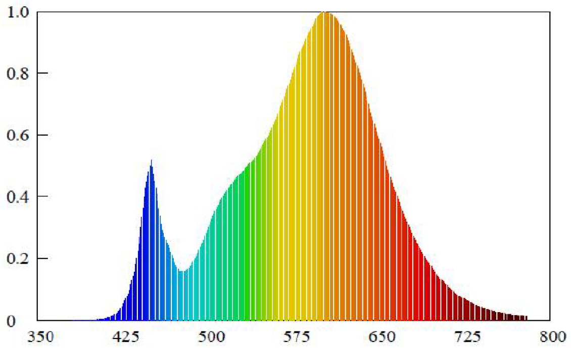
Spectral power distribution (3000K)
