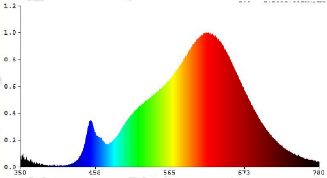
WE-SL1502W
