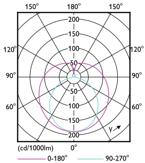
Light Distribution Diagram - MAS LEDtube VLE 1500mm UE 22.1W 840 T8
