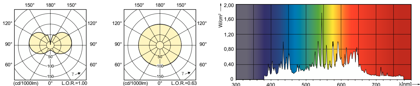
Light Distribution Diagram - MASTERColour CDM-E MW eco 360W/842 E40
