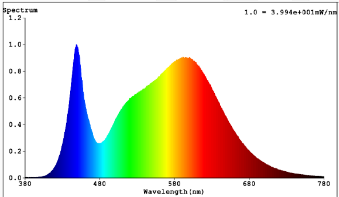
Spectral power distribution for light source of SSL-TPL-18W-230V 4000K:
